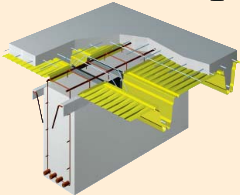
Hoesch Additive Floor® on precast concrete girder
